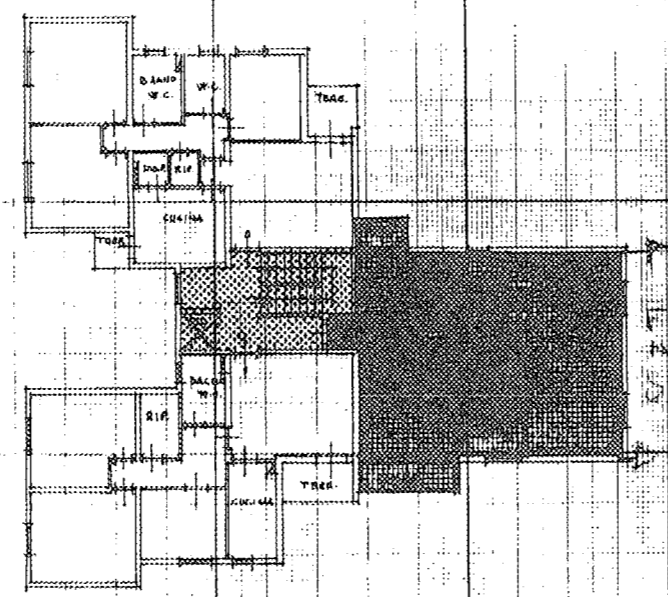
PIANO QUARTO H=2.70
