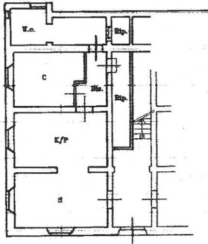
PIANO TERRA H= 3.96
